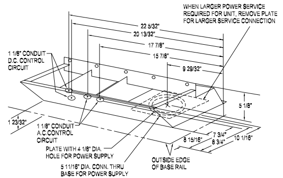
DETAIL "B" COVERS 40, 60, 70 AND 75 TON UNITS
